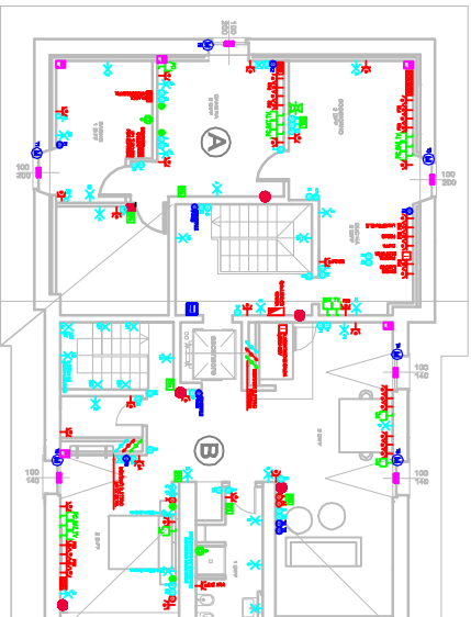
PIANO MANSARDATO
